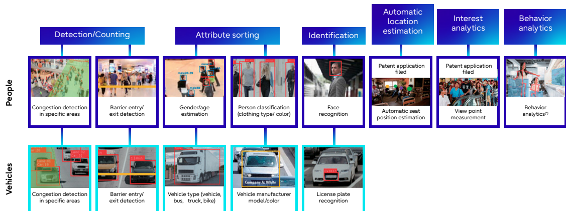
Fig. 1 - Functionality of GREENAGES Citywide Surveillance, Fujitsu's AI video analysis solution
